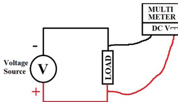
FIGURE 66: DC Voltage measurement on multi-meter 67
