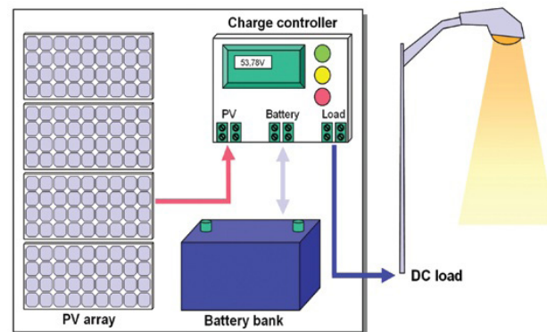
FIGURE 33: Standalone DC Power System 34
