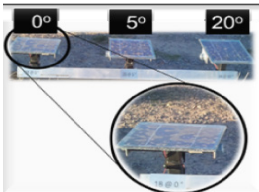
FIGURE 60: Effect of Tilt Angle on Soiling Loss 61
