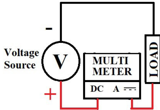
FIGURE 67: DC current measurement schematic 68
