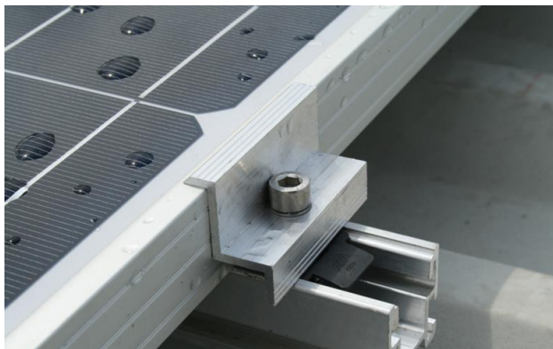
FIGURE 52: Mounting Fixture 53
