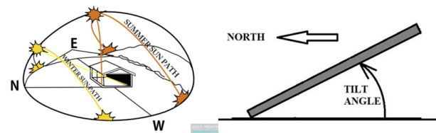
FIGURE 4: Path of the Sun during the year 4 and solar panel tilt 5
