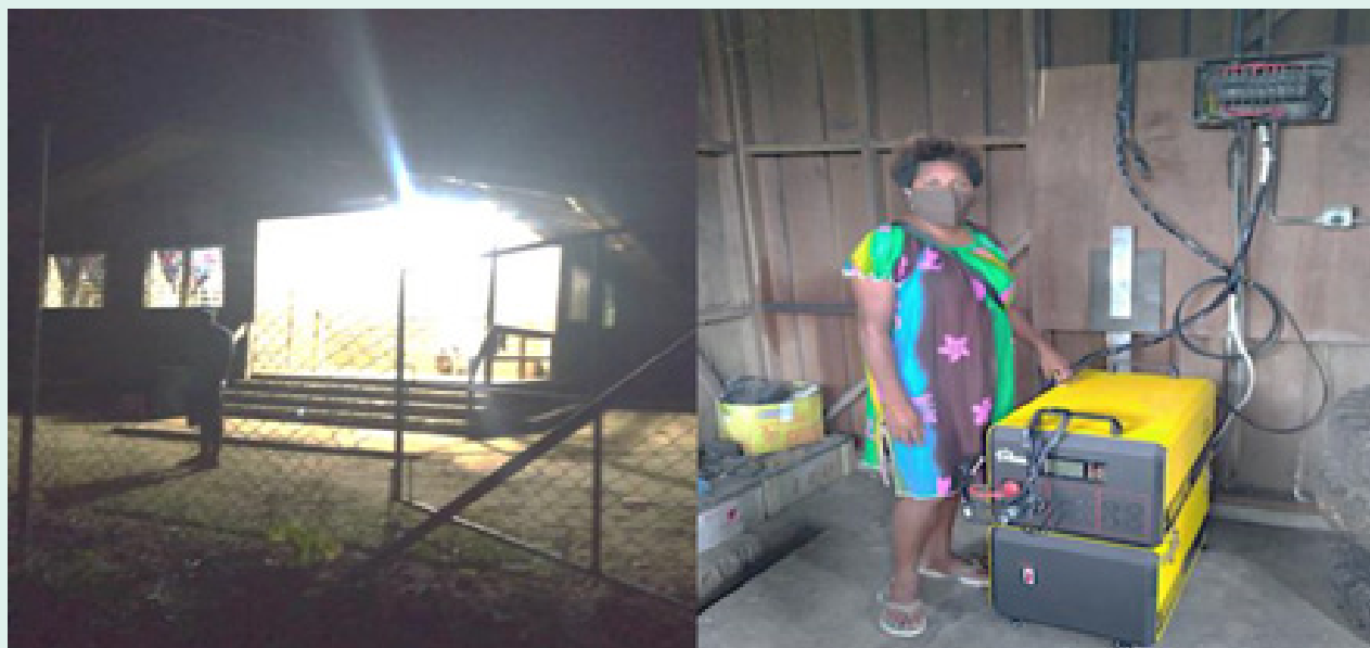
FIGURE 38: Installation of mini-grid solar powered station at Kikori Police Station & Lights at Night, (left) Mini-grid solar Power station Storage room with switch board-Kikori (right) 39
