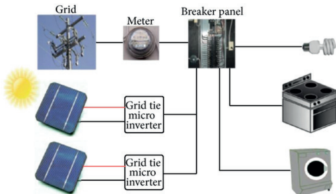
FIGURE 35: Grid connected Solar PV System 36
