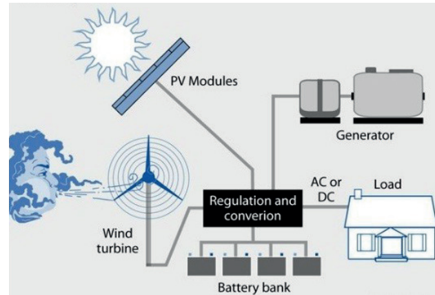
FIGURE 36: Wind Solar Hybrid System 37
