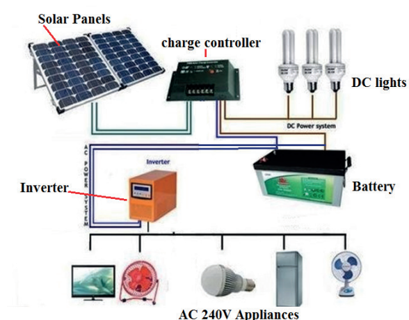
FIGURE 34: Standalone AC/DC Power System 35
