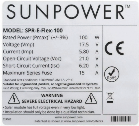
FIGURE 57: Nameplates 60
