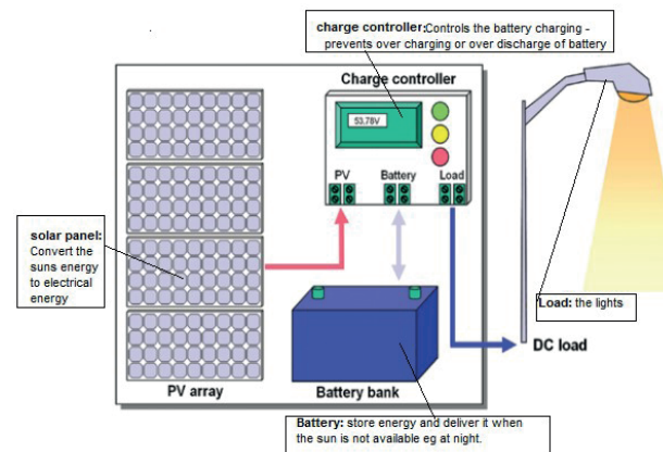
FIGURE 33: Standalone Power System 34
