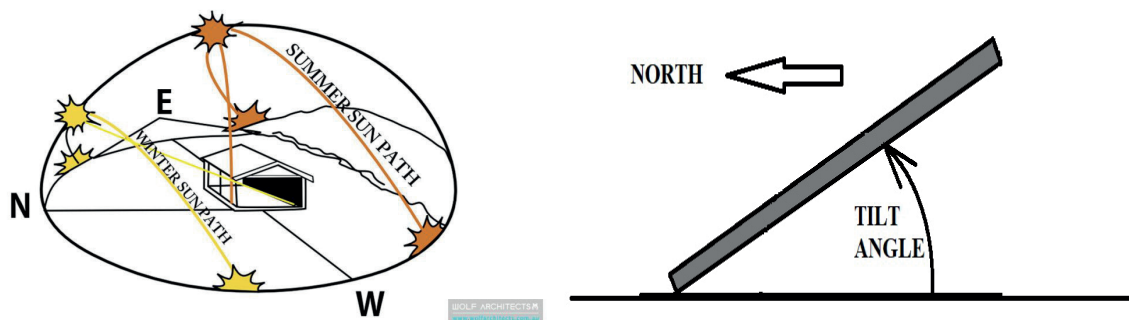
FIGURE 4: Path of the Sun during the year 4 and solar panel Tilt 5
