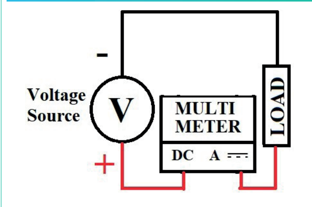
FIGURE 68: DC current measurement on multi-meter 71
