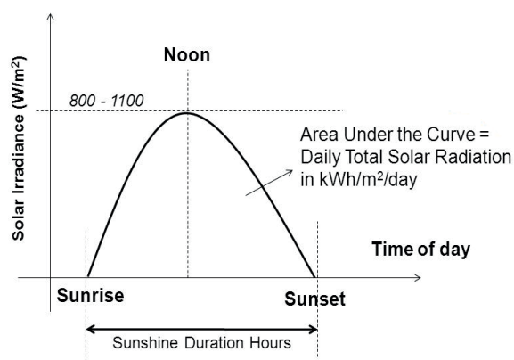
FIGURE 3: Solar Irradiance Graph 3
