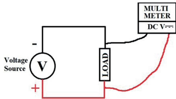
FIGURE 66: DC Voltage measurement on multi-meter 69
