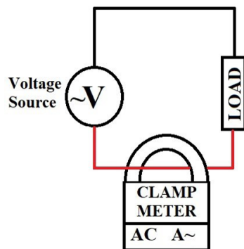
FIGURE 55: AC current measurement schematic 65
