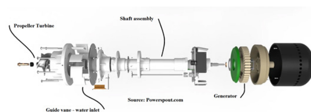
FIGURE 26: Propeller Turbine Generator (Exploded view) 36
