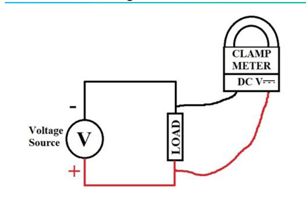
FIGURE 48: DC Voltage measurement on clamp meter 58
