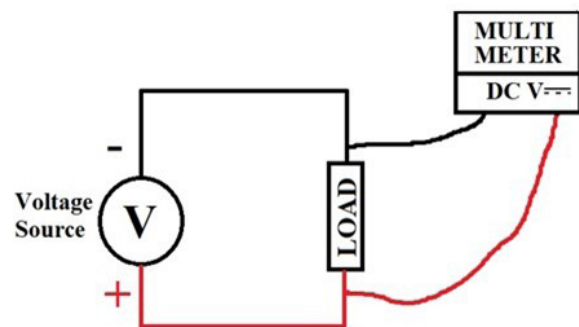
FIGURE 58: DC Voltage measurement on multi-meter 68
