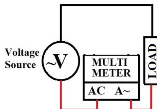
FIGURE 66: AC current measurement on multi-meter 76
