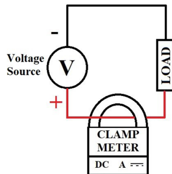
FIGURE 53: DC current measurement schematic 63
