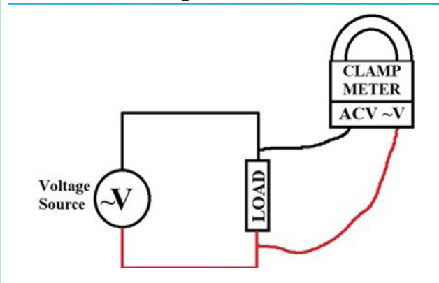
FIGURE 50 : AC Voltage measurement on clamp-meter 60
