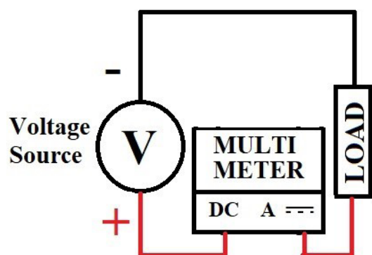
FIGURE 63: DC current measurement schematic 73
