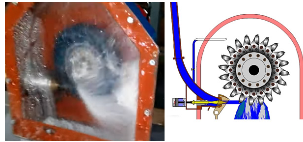
FIGURE 27: Water forcing a Pelton Turbine to rotate 37
