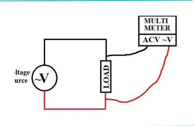
FIGURE 60: AC Voltage measurement on multi-meter 70
