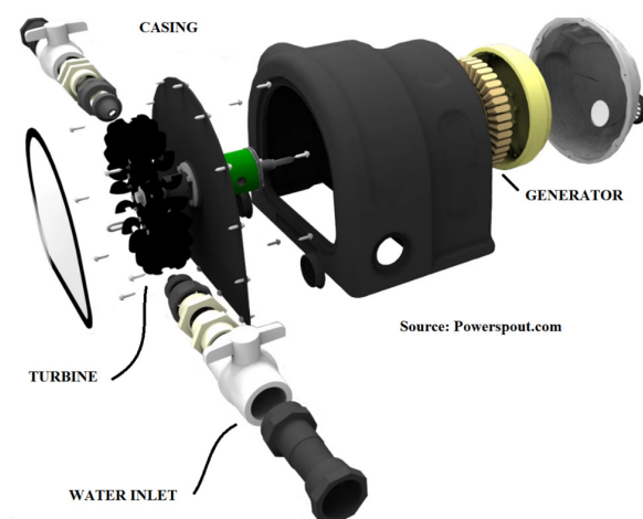
FIGURE 25: Pelton Turbine Generator (Exploded view) 35
